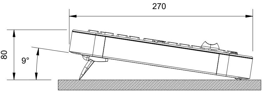
SIDE VIEW (LEFT) : T3 CONSOLE (PROPPED)
