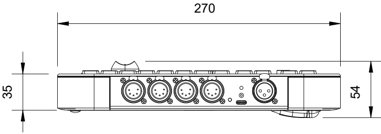
SIDE VIEW (RIGHT) : T3 CONSOLE
