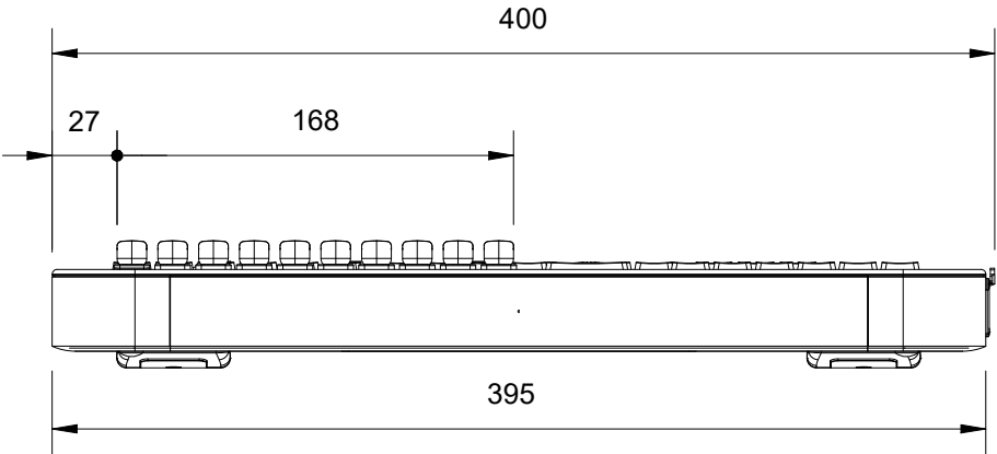
FRONT VIEW : T3 CONSOLE
