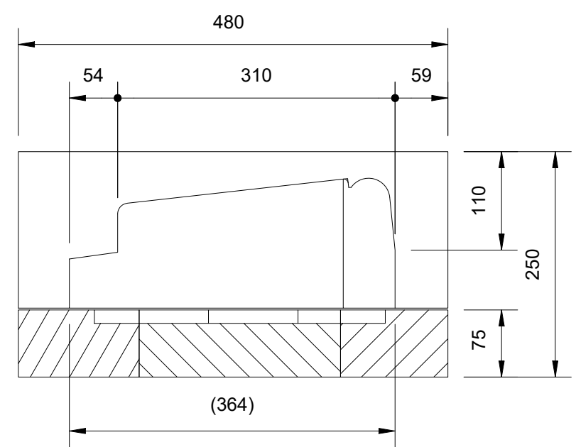
SECTION VIEW B-B ( SCALE 1 : 6 )
