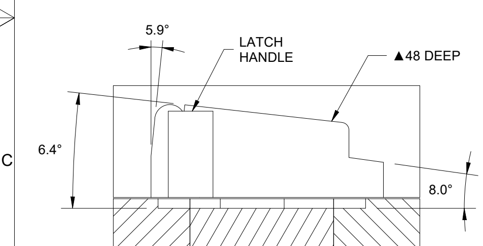
SECTION VIEW A-A ( SCALE 1 : 6 )
