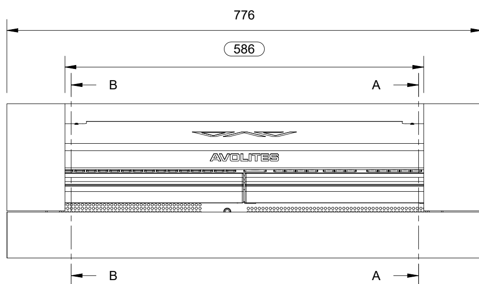
FRONT VIEW : D7-215 CONSOLE : CASE FOAM ( SCALE 1 : 6 )
