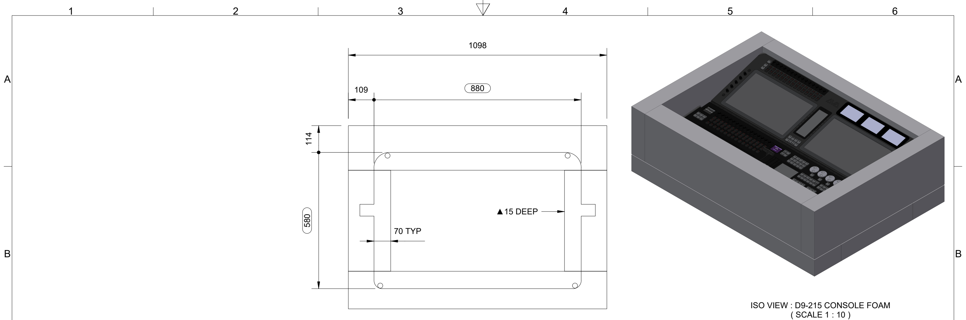
TOP VIEW : D9-215 CONSOLE : BASE FOAM ONLY ( SCALE1 : 10 )
