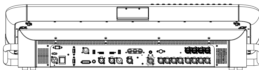
REAR VIEW 'A' : D9-215 CONSOLE
