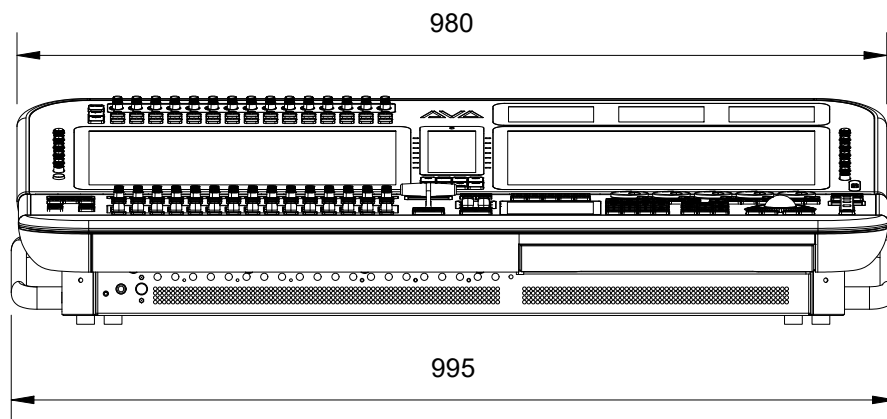
FRONT VIEW : D9-215 CONSOLE (SCREEN DOWN)
