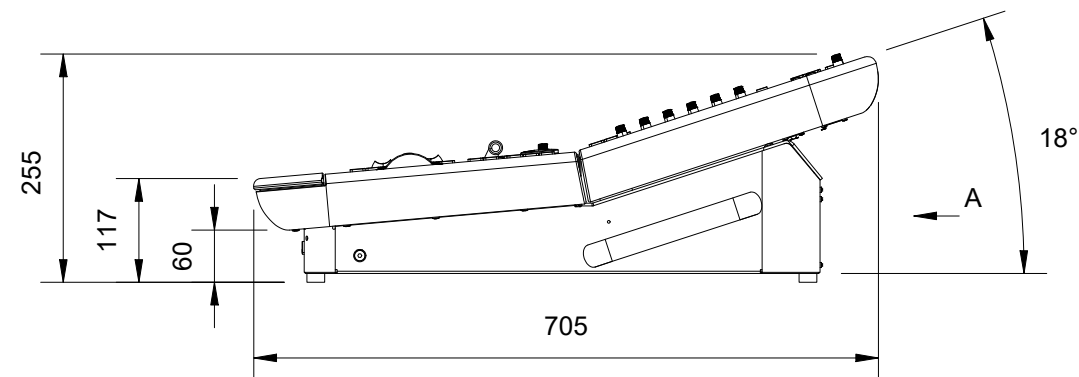
SIDE VIEW (RIGHT) : D9-215 CONSOLE (SCREEN DOWN)
