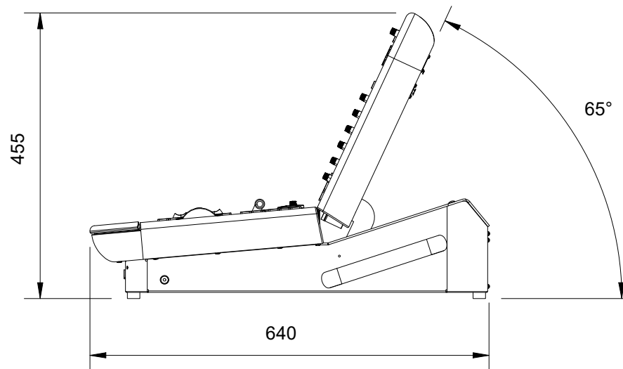
SIDE VIEW (RIGHT) : D9-215 CONSOLE ( SCREEN UP )
