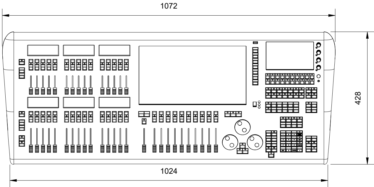
TOP VIEW: ARENA CONSOLE
