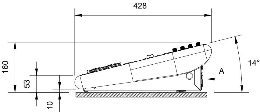
SIDE VIEW (RIGHT) : ARENA CONSOLE
