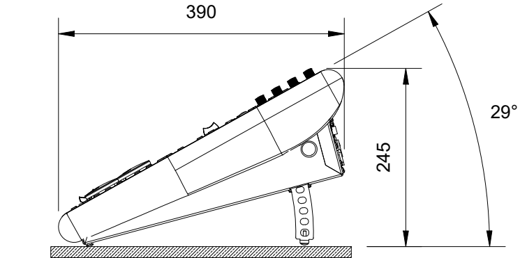
SIDE VIEW (RIGHT) : ARENA CONSOLE (PROPPED)
