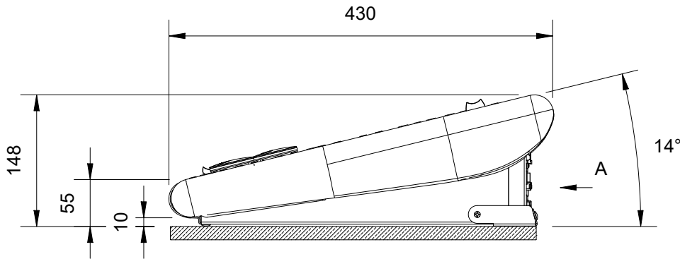
SIDE VIEW (RIGHT) : TIGER TOUCH II CONSOLE
