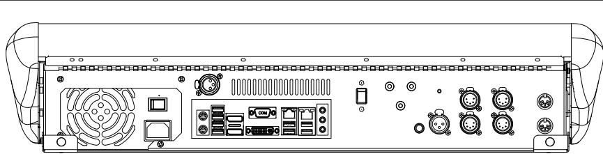
REAR VIEW 'A' : TIGER TOUCH II CONSOLE
