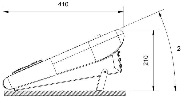
SIDE VIEW (RIGHT) : TIGER TOUCH II CONSOLE (PROPPED)
